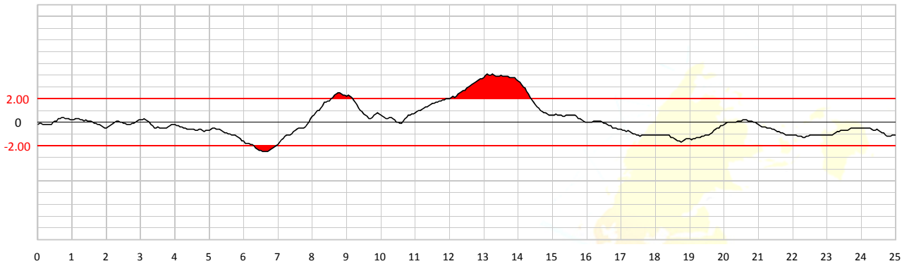
1m Gauge
